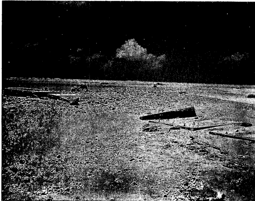
Fig. 10—Posttest view of two-way slabs at station 360.01, range 1830 ft, looking away from GZ, showing evidence of foundation failure.
